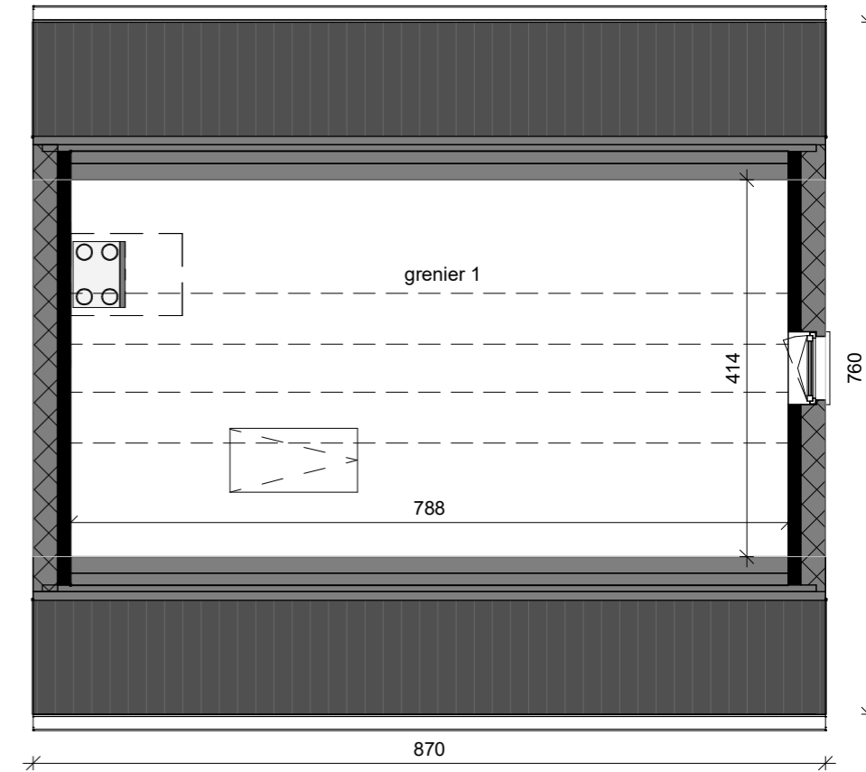
grenier surf. brute 36.02 m 2
